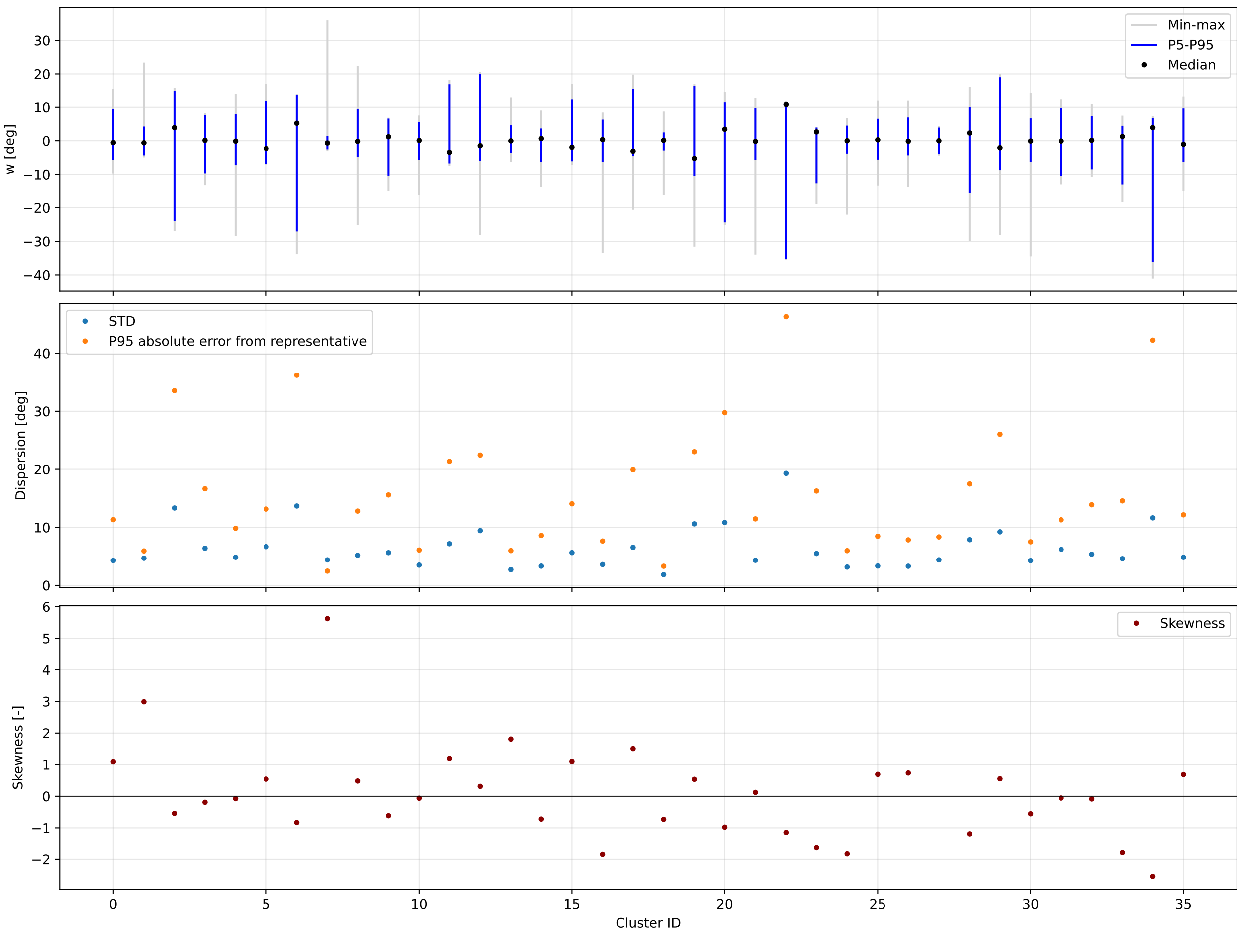
K=36 | backward | w | valid=194124/194124 | offsets from each cluster circular mean
