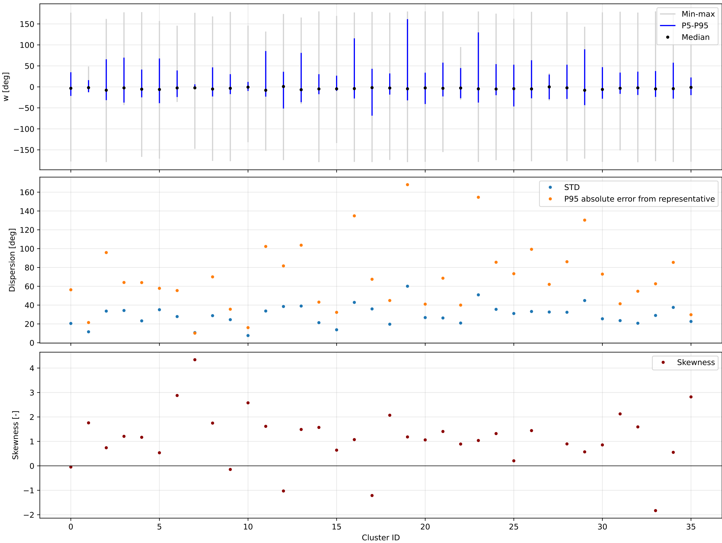
K=36 | forward | w | valid=194058/194124 | offsets from each cluster circular mean
